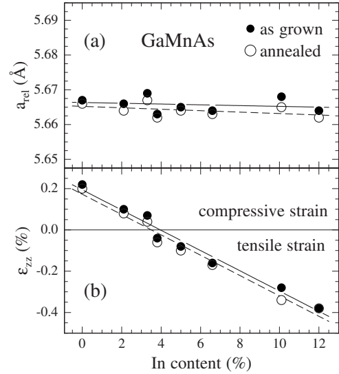
FIG. 4. (a) Relaxed lattice parameter a_{\text{rel}} and (b) vertical strain \varepsilon_{zz} of the (Ga,Mn)As layer plotted against the In content in the (In,Ga)As buffer. Postgrowth annealing only leads to a slight decrease of the values.
