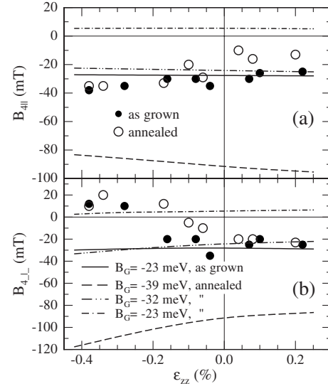
FIG. 10. Dependence of the cubic anisotropy parameters (a) B_{4\parallel} and (b) B_{4\perp} on \varepsilon_{zz} for the as grown (solid circles) and annealed samples (open circles). The lines are model calculations within the microscopic theory using the same values for p and B_G as in Fig. 8(b).
