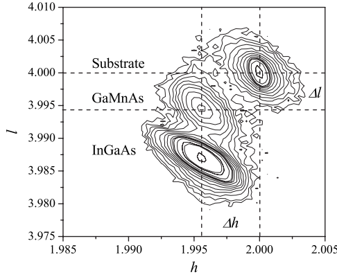
FIG. 2. Reciprocal space map around the asymmetric (224) reflections of a nearly unstrained (Ga,Mn)As layer ( \varepsilon_{zz} = -0.04\% ) grown on relaxed (In,Ga)As/GaAs template. h and l are the coordinates in k space in units of the reciprocal-lattice vectors along [100] and [001] in the GaAs substrate, respectively. \Delta h and \Delta l denote the shift of the peak position relative to that of the substrate. In the plot, \Delta h and \Delta l are only depicted for the (Ga,Mn)As layer.
