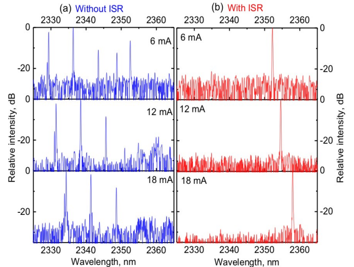
Fig. 3: Emission spectra of the VCSEL at different driving currents. device (a) before and (b) after applying an ISR
