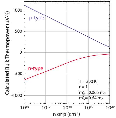
FIG. 1. (Color online) Calculated carrier concentration dependence of the thermopower at 300 K of n- and p-type InN using Eq. (1).
