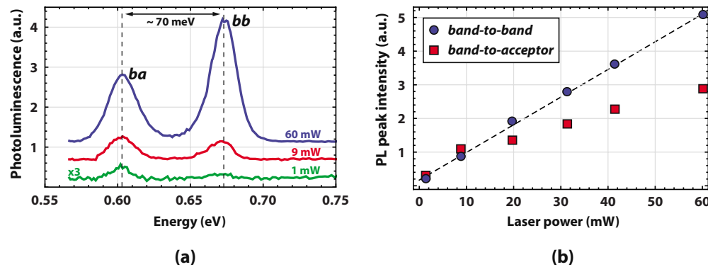
FIG. 5. (Color online) (a) PL spectra at \sim 25 K of the sample with the lowest Mg content, 101107C ( S_{300\text{ K}} = -206 \mu\text{V/K} ), for several different laser excitation intensities, vertically offset for clarity. Two peaks are clearly resolved: one associated with band-to-band emission ( bb ), the other with band-to-acceptor transitions ( ba ) as explained in the text. (b) Peak PL intensity is plotted as a function of pumping laser power. The dashed line in (b) is a linear fit to the bb data.
