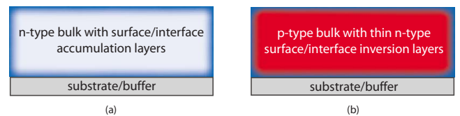
FIG. 2. (Color online) (a) Illustration of n-type InN with surface and interface accumulation layers (blue), (b) illustration of p-type InN with p-type bulk (red) and surface/interface inversion layers (blue). The inversion and accumulation layer thicknesses are exaggerated here; in reality the surface layers are on the order of 10 nm thick while the films are on the order of 0.5 to 1 \mu\text{m} thick.
