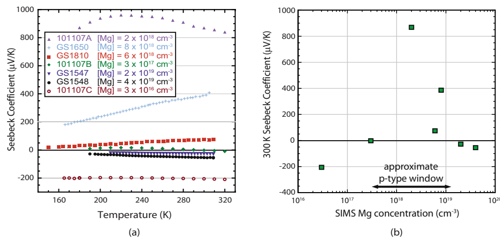
FIG. 3. (Color online) (a) Measured Seebeck coefficient of Mg-doped InN samples as a function of temperature. SIMS Mg content shown in legend. (b) Measured Seebeck coefficient of Mg-doped InN samples at room temperature as a function of the Mg concentration measured by SIMS.
