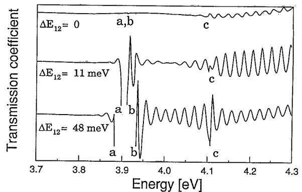
FIG. 15. Transmission coefficient for tunneling from the valence bands into the conduction bands shown in Fig. 14, plotted as a function of the outgoing conduction band electron energy, for k_{\parallel} = 0 . The letters a, b, c refer to the energy band positions specified in Fig. 14. The figure illustrates the suppression of the WS resonances with diminishing conduction band splitting \Delta E_{12} .
