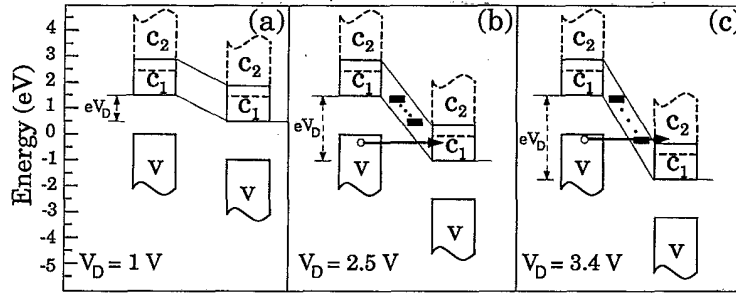
FIG. 9. Schematic band picture of a GaAs p-i-n diode, illustrating the origin of Wannier-Stark resonances in the Zener tunneling current. (a) No WS resonances form when the potential drop is smaller than the first conduction band width \Delta_{c1} . In addition, there is no Zener tunneling in this case since V_D < E_{\text{gap}} . (b) When V_D exceeds the first conduction band width, one obtains WS resonances of finite width that are associated with the first conduction band (thick bars). The WS resonances do not overlap in energy with the extended semibulk states associated with the first conduction band in the right region and, therefore, cannot contribute to the (elastic) Zener tunneling current. (c) For V_D = 3.4 V ( eV_D > E_{\text{gap}} + \Delta_{c1} ), WS states resonantly enhance the tunneling current from the valence band to the second conduction band and produce oscillations in the current as a function of V_D .
