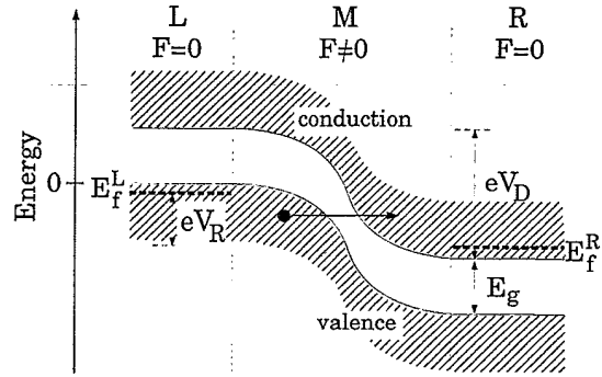
FIG. 2. Schematic picture of the tilted electronic band edge states in a typical p - n or p - i - n junction with a high electric field. The total potential drop ( V_D ) is defined as the potential difference between the left and right semibulk region ( L, R ). The reverse bias ( V_r ) is the difference between the Fermi levels in the L and R regions. High n and p doping ensures that the field is nonzero only in the M region. In this and all following figures, the zero of energy lies at the top of the valence band in the left ( p -doped) semibulk region.
