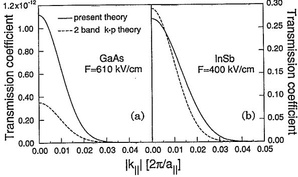
FIG. 10. Calculated energy-averaged Zener tunneling coefficient for (a) a GaAs and (b) an InSb p - i - n diode (20 nm i zone) as a function of |k_{\parallel}| . The electric fields F are indicated in the figure. The present full-band multichannel results are compared to the widely used two-band \mathbf{k} \cdot \mathbf{p} model of Kane (Ref. 24). The high value of the transmission coefficient in InSb originates in the small band gap.
