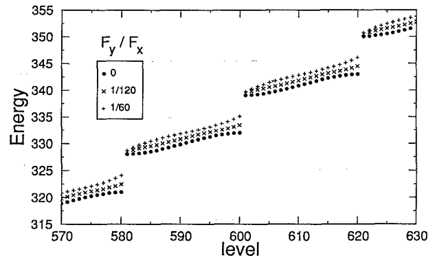
FIG. 16. Energies of a two-dimensional one-band tight-binding Hamiltonian in a constant electric field \mathbf{F} with components F_x and F_y , in units of t . The figure shows a representative part of the spectrum. The lattice consists of 60 and 20 sites in the x and y directions, respectively. The WS levels do not change qualitatively with the direction of the electric field, even when \mathbf{F} points to the lattice vector F_y/F_x = 1/60 , provided the potential drop in the y direction is smaller than the band width.
