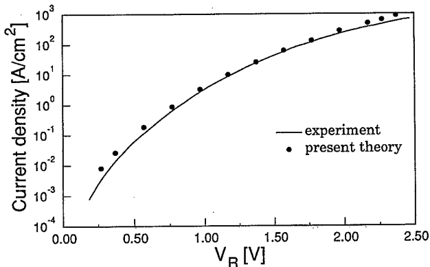
FIG. 11. Comparison between the experimental and calculated tunneling current density as a function of the reverse bias for a GaAs p - i - n structure with an 18nm i zone, and doping concentration of n=10^{19} \text{ cm}^{-3} and p=2 \times 10^{19} \text{ cm}^{-3} .
