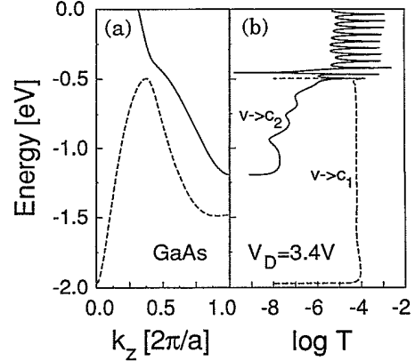
FIG. 4. (a) Energy band structure of first and second conduction bands along the [001] direction. (b) Calculated transmission coefficient for same p - i - n structure as in Fig. 3, summed over all in-channel states associated with hole bands and for V_D = 3.4 \text{ V} . The out-channel states are associated with either the first ( c_1 ) or second ( c_2 ) conduction band. The logarithm is to base 10.
