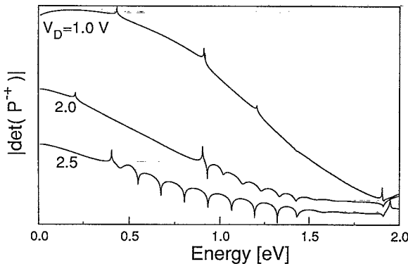
FIG. 8. Calculated determinant of the transfer matrix element \mathbf{P}^{-+} as a function of energy for a GaAs p - i - n structure with an intrinsic zone of 5.4 nm width and for \mathbf{k}_{\parallel} = \mathbf{0} . The equally spaced minima in the determinant reflect the presence of WS resonances associated with the first conduction band and appear for V_D > \Delta_{c1} .
