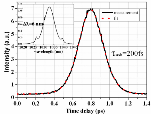
Fig. 3. (Color online) The autocorrelation and the spectrum (inset) at 17 W of output power and 5.5% output coupler (measured with an APE Pulse Check autocorrelator). The time-bandwidth product is 0.34 ( \text{sech}^2 , ideal 0.315). Kelly sidebands are visible in the spectrum wings. This measurement was performed for the SESAM-assisted KLM.
