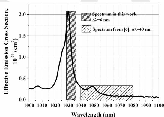
Fig. 1. The emission spectrum of Yb:YAG gain medium. The shaded areas show the spectra (FWHM) generated in the present work and in [6]
