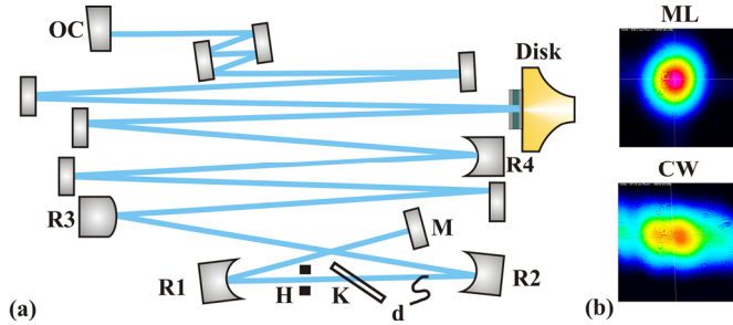
Fig. 2. (Color online) a): Schematic of the KLM Yb:YAG disk oscillator. All flat mirrors except for M are high-dispersion mirrors with \approx 1200 \text{ fs}^2 per bounce; OC, an output coupler with 5.5% or 14% transmission; R1, R2 concave mirrors with 0.3 m radius of curvature; R3, -4 m; R4, 4 m; K, 1-mm-thick fused silica plate placed in the focus at the Brewster angle; H, hard aperture (a pinhole); M flat mirror or SESAM. The pulse repetition rate is 40 MHz. The oscillator is placed inside a box of size 1 \times 0.4 \text{ m}^2 . b): the beam profile in mode-locked regime and in CW regime (after mode-locking has been interrupted).
