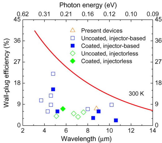
Fig. 4. Comparison of overall efficiency for injector-based (blue, squares) and injectorless devices (green, diamonds) around 300 K. The efficiency of the present devices is given by an orange triangle. The solid theoretical line of efficiency versus wavelength is taken from reference [8].
