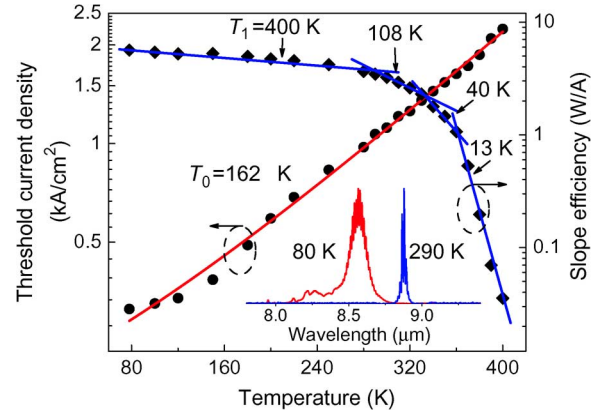
Fig. 2. Threshold current density and slope efficiency versus temperature for an as-cleaved 4-mm-long and 30- \mu\text{m} -wide laser. Characteristic temperatures T_0 for j_{\text{th}} and T_1 for slope efficiency are shown. The inset shows the normalized emission spectra at 80 K and 290 K.
