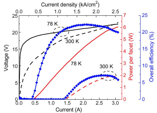
Fig. 3. Optical output power per facet, voltage, and overall efficiency over current for a 4-mm-long and 30- \mu\text{m} -wide device. The voltage is given by the black solid (78 K) and dashed (300 K) lines, while the output power is given by the red solid (78 K) and dashed (300 K) lines. The overall efficiency is indicated by blue scatters.
